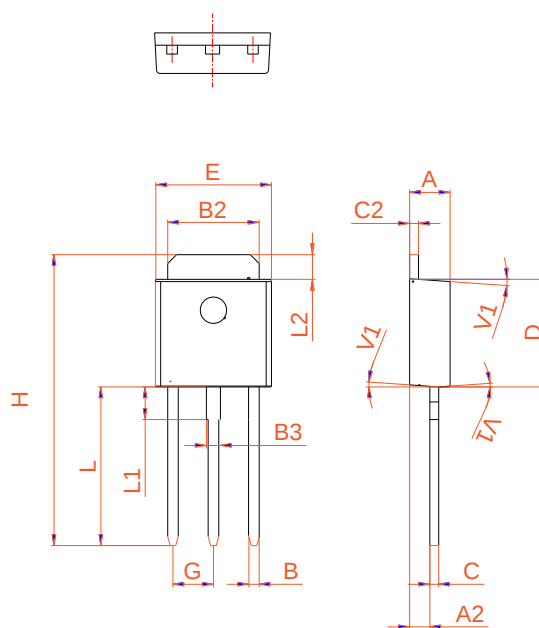
TO-251
